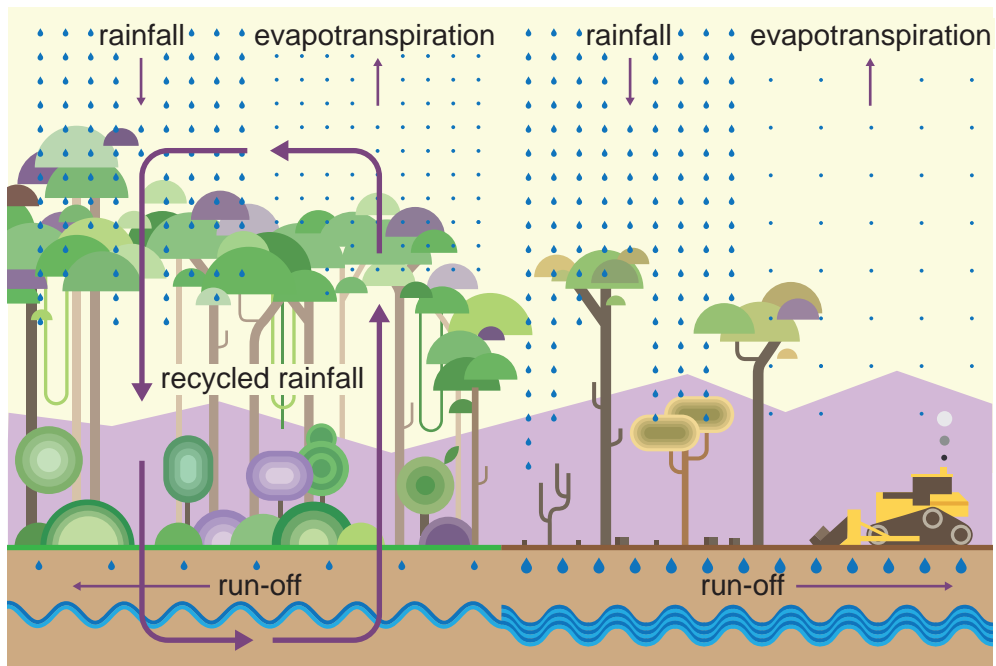
Fig. 2 – Tropical rainforest water cycle.
