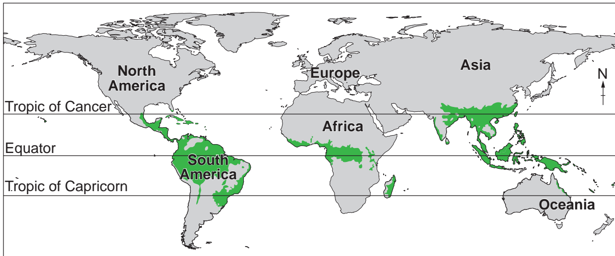
Fig. 1 – Global distribution of tropical rainforests.
